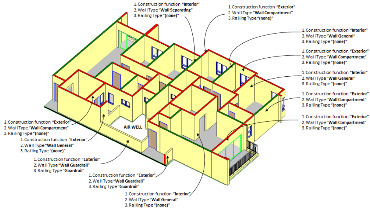
Figure 4 "Wall Type" Parameter Settings
