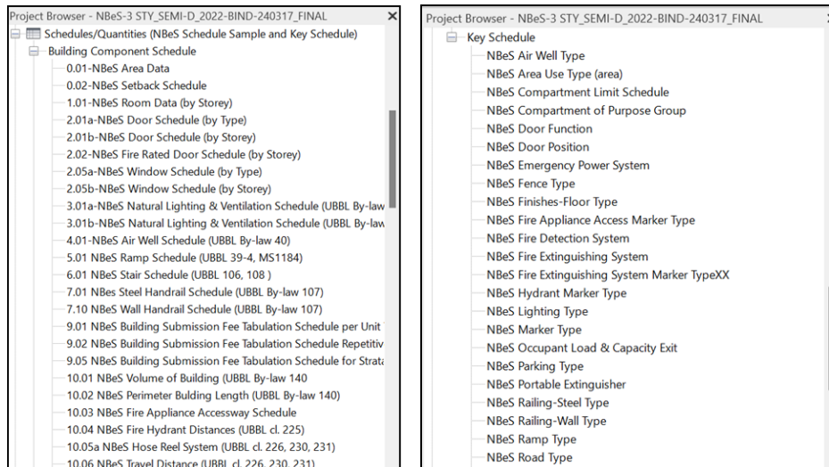
Figure 3 NBeS Project Browser
